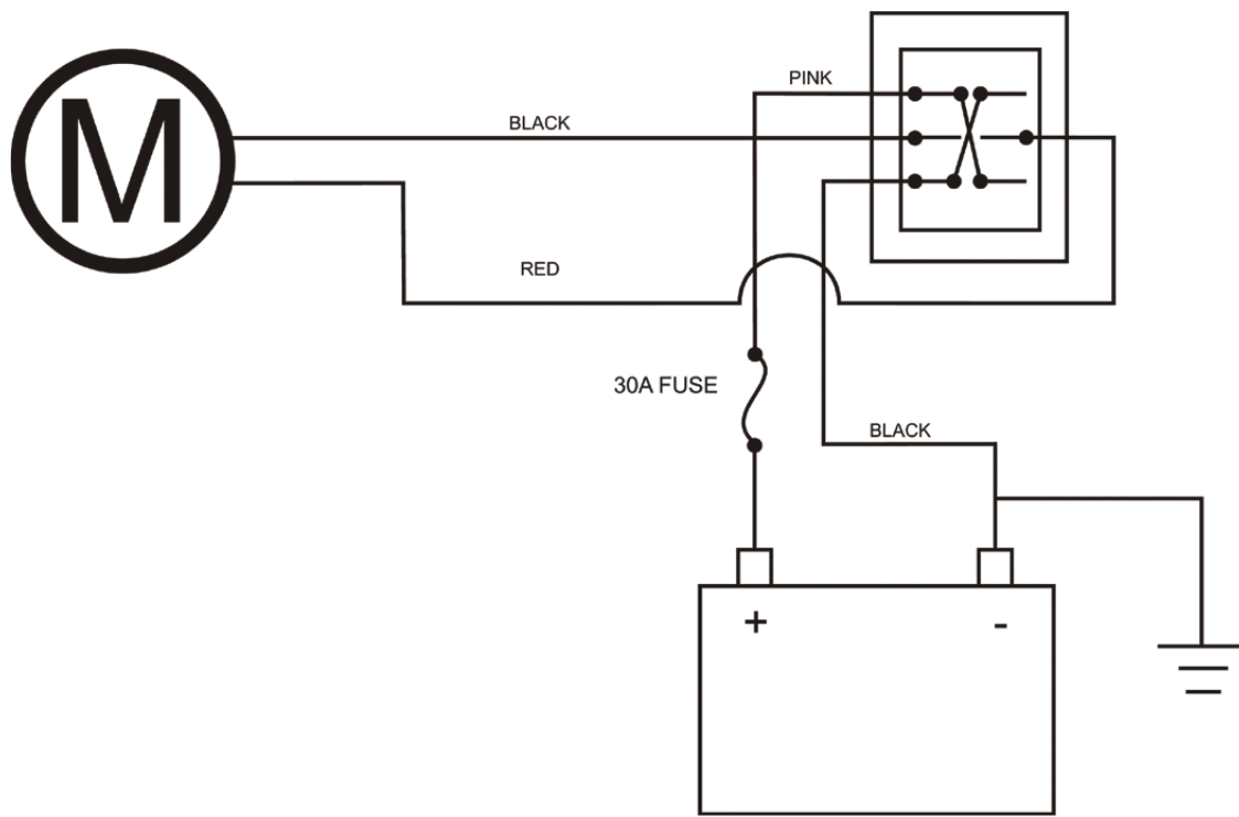
ELG SWITCH WIRING DIAGRAM
